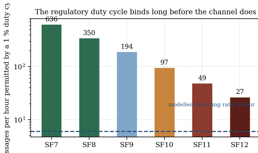
Fig.6: Messages per hour permitted by the regulatory duty cycle, on a logarithmic scale.
