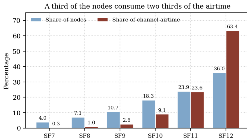
Fig.2: Share of nodes against share of channel airtime, by spreading factor.
