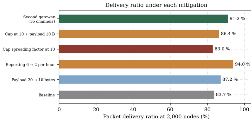
Fig.4: Delivery ratio under each mitigation.
