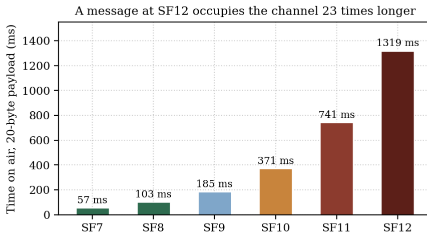
Fig.1: Time on air for a 20-byte payload at each spreading factor.
