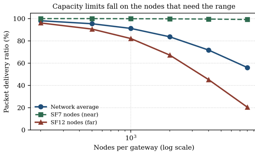
Fig.3: Packet delivery ratio against node count for the network and for the two extreme spreading factors.
