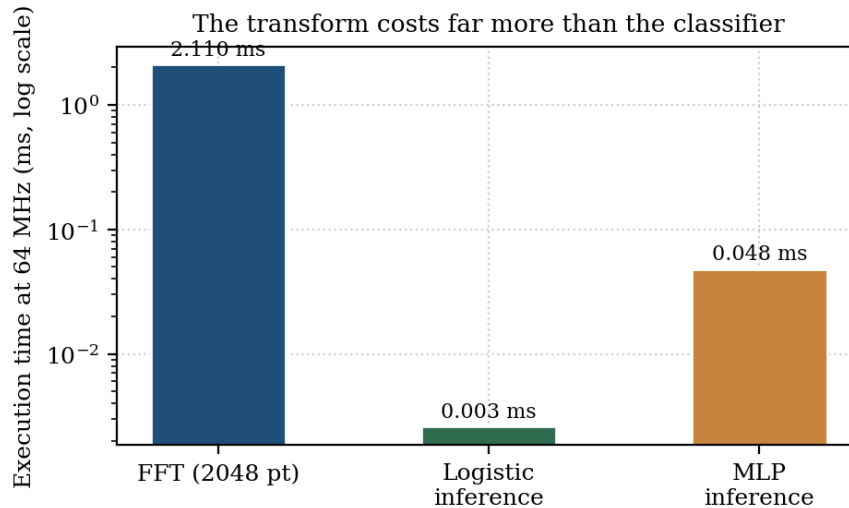
Fig.5: Execution time of each processing stage at 64 MHz, on a logarithmic scale.
