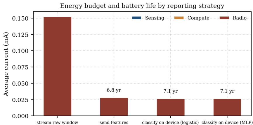
Fig.4: Average current decomposed into sensing, compute and radio, with battery life annotated.
