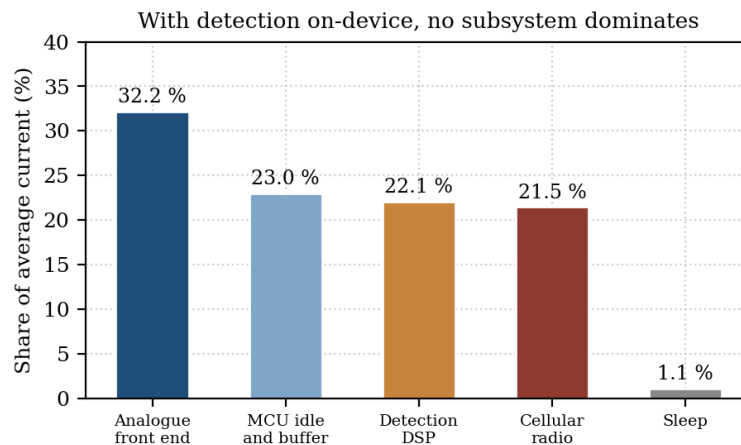
Fig.4: Energy budget of the on-device detection design.
