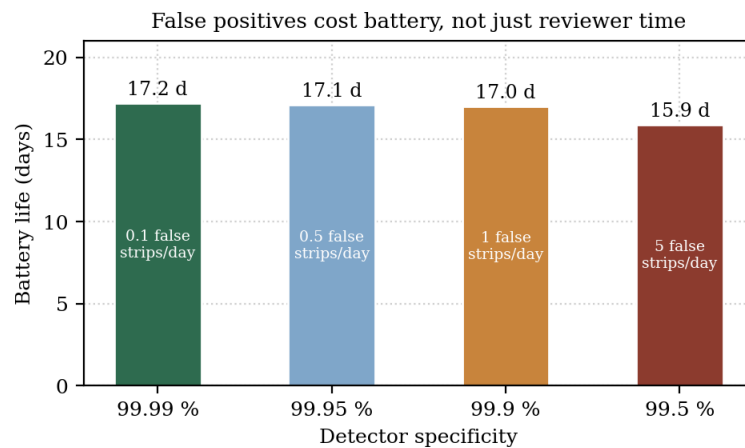
Fig.6: Recording duration against detector specificity.
