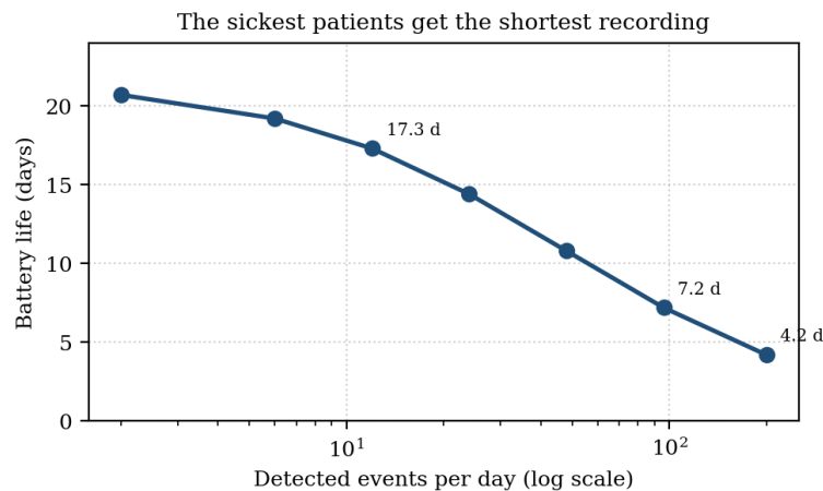
Fig.5: Recording duration against the number of events detected per day.
